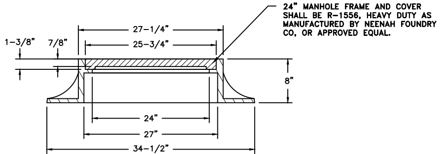
24" MANHOLE FRAME AND COVER
