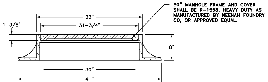
30" MANHOLE FRAME AND COVER
