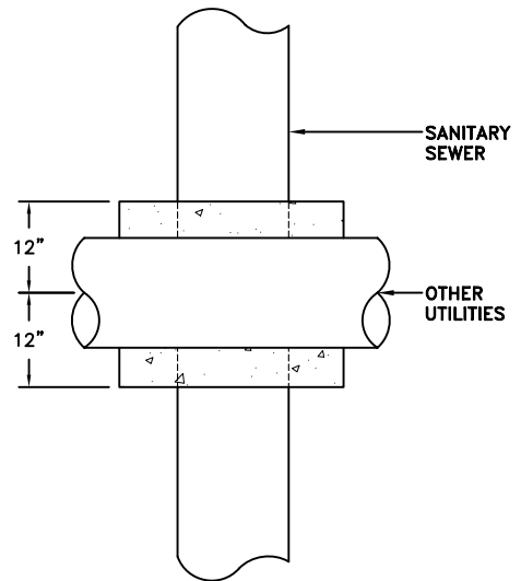
UTILITY CROSSINGS
