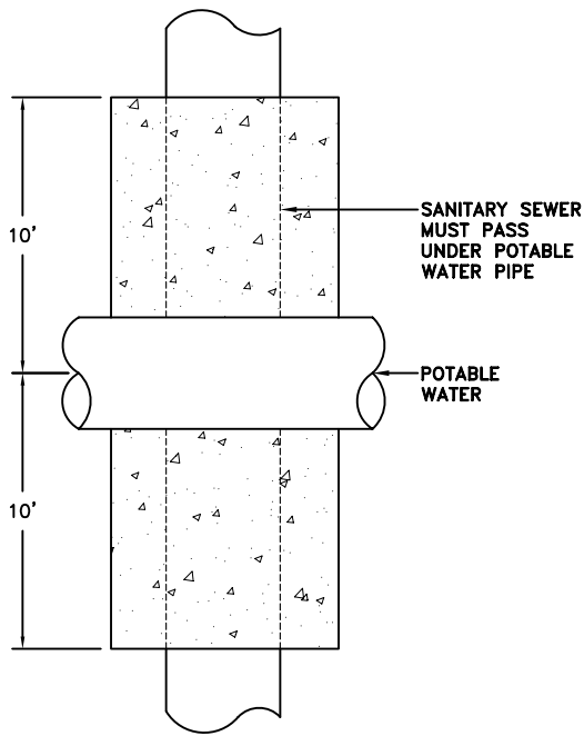
WATER CROSSINGS
